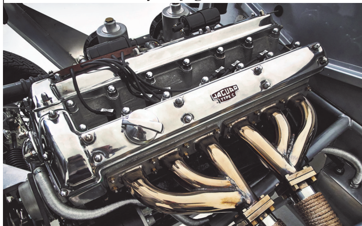
The 3.4 Litre C (competition) engine with SU Carburettors
